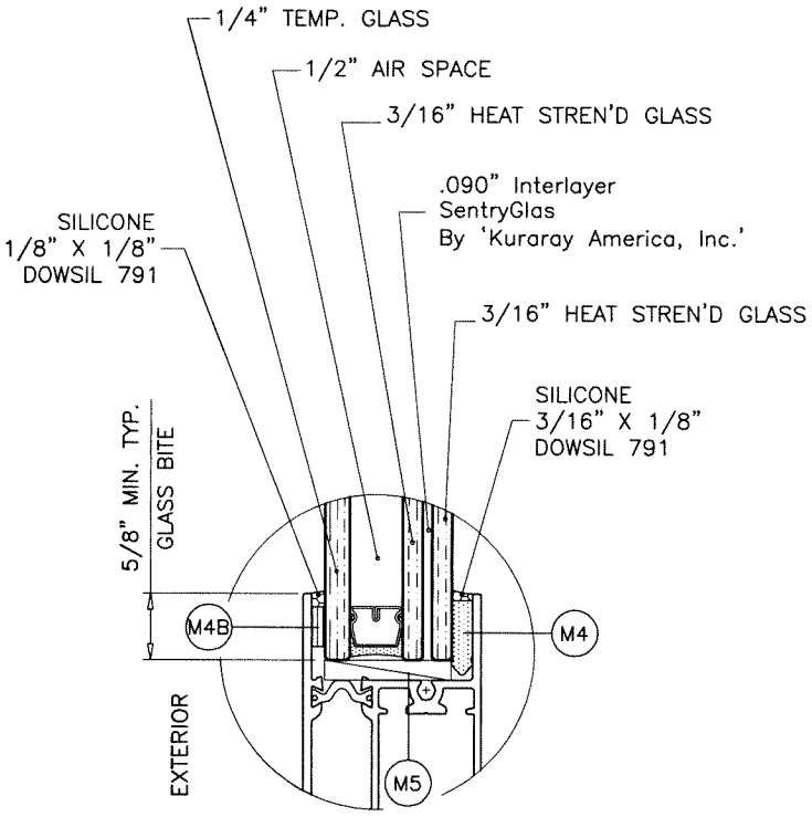
GLASS TYPE 'GL1' 1-1/4" OVERALL INSUL. LAM. GLASS
